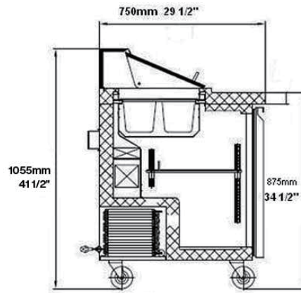
Section View
